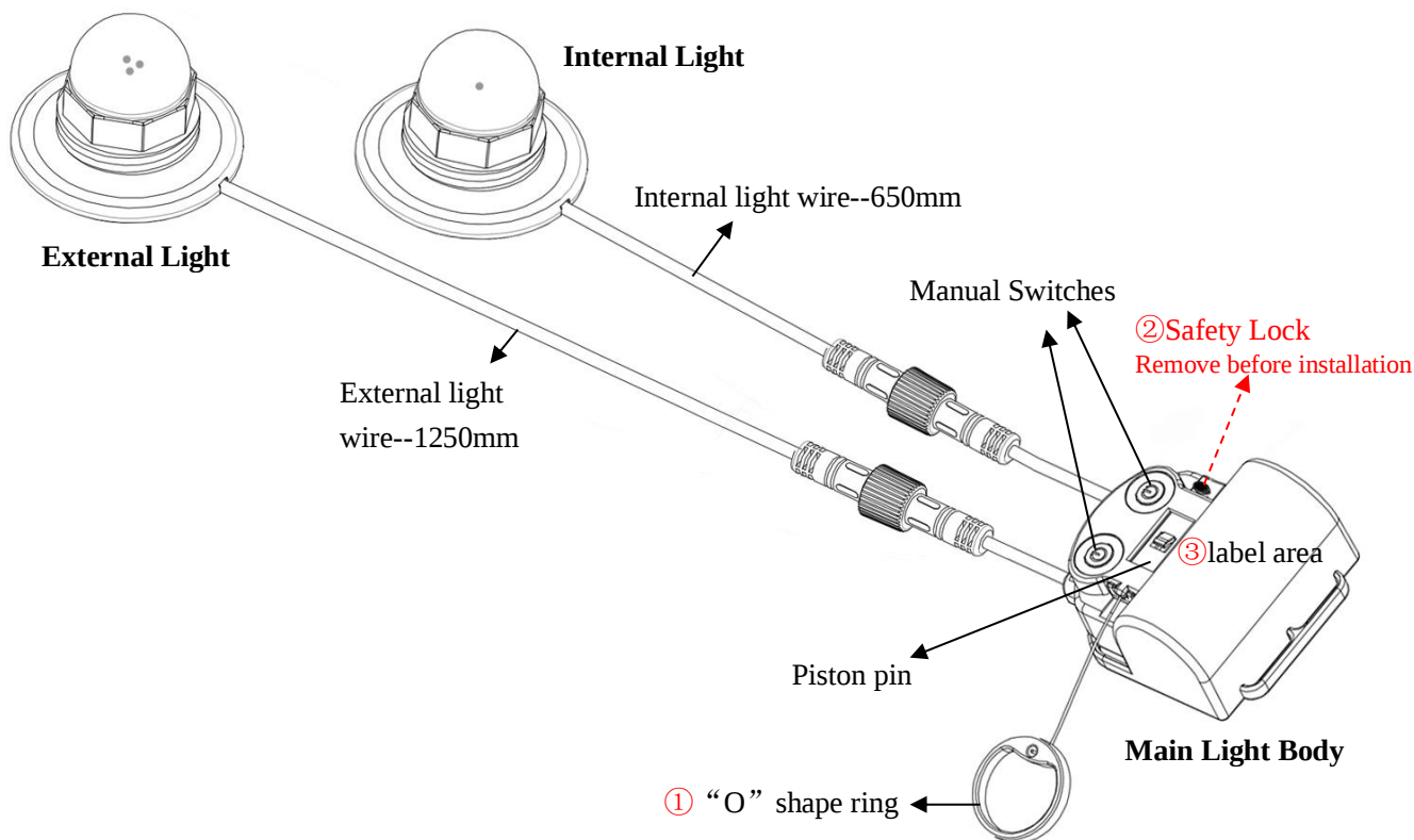
Figure 2-1 Product Structure
